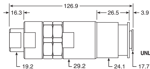
UNLOADED #10 AUTO-LOAD GAGE SET AT MINIMUM
