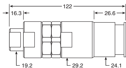
UNLOADED #10 GAGE SET AT MINIMUM
