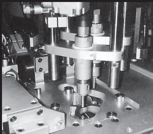
TITAN LANCER® -1 Drivers with Machine Load Stud Retainers. Stud projection height controlled by spindle stops.
