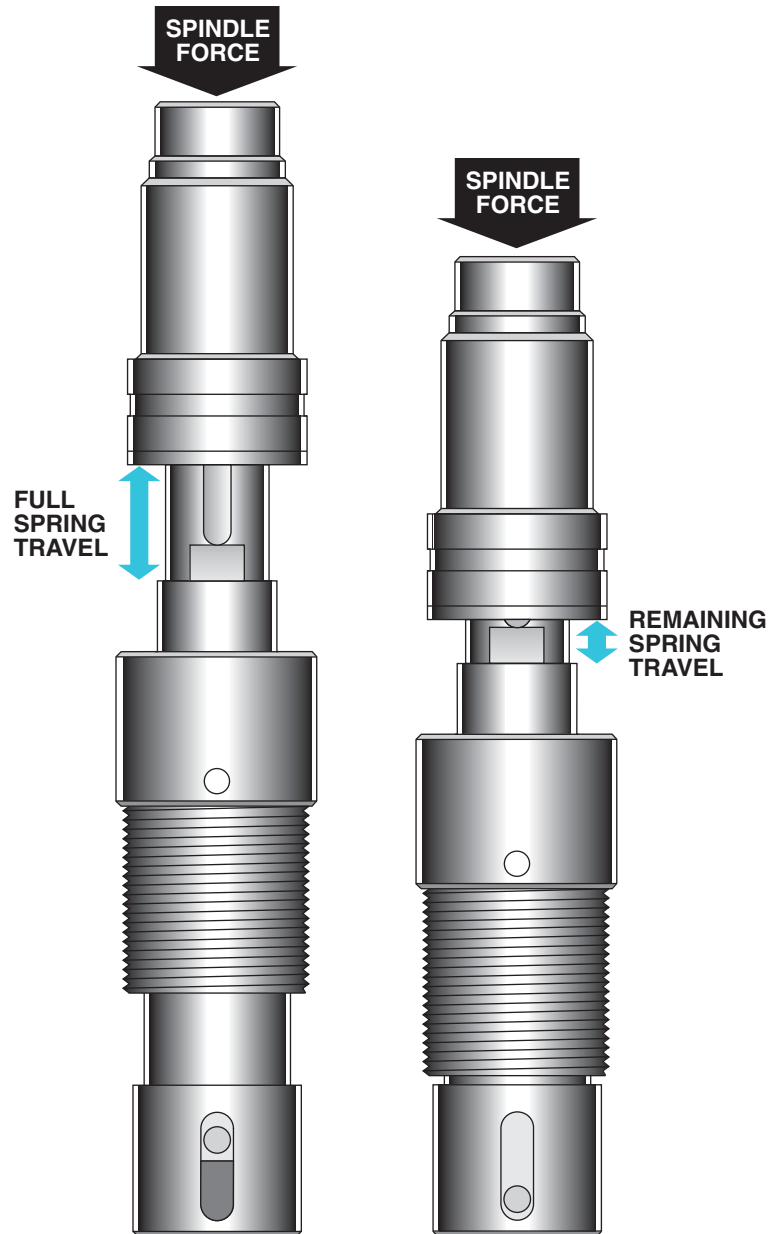
Lancer #2 shown with TTSL-1.
